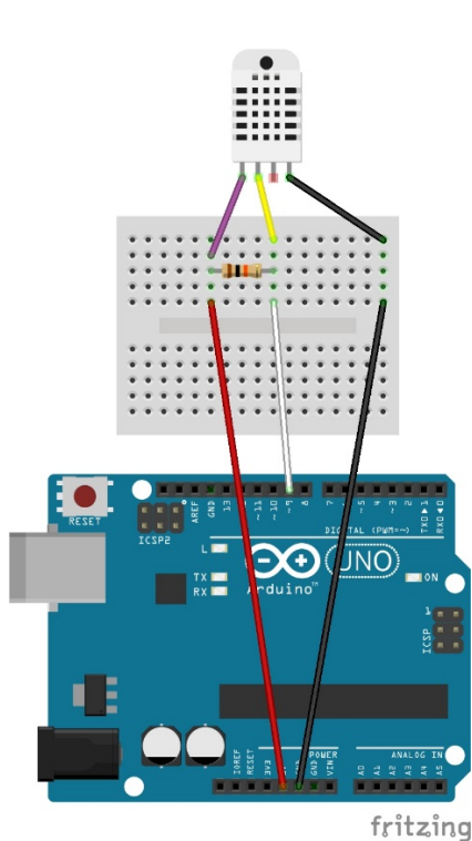
Figure 4. Wiring diagram for DHT22 and Arduino
